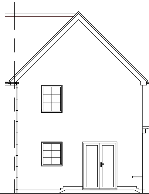
SIDE ELEVATION
